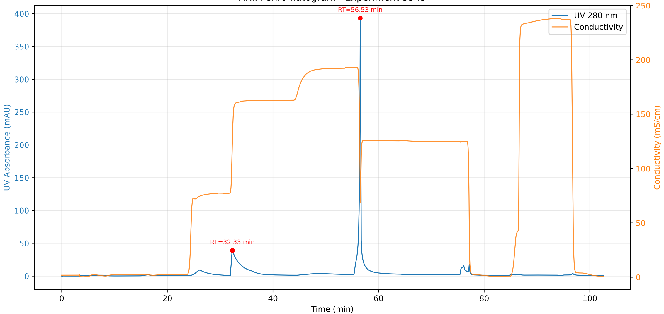
AKTA Chromatogram - Experiment 5545
